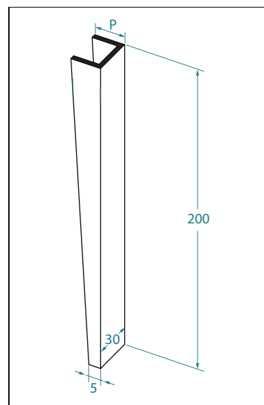
PROFILO CONICO - L 30 mm TAPERED PROFILE - L 30 mm
