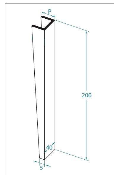
PROFILO CONICO - L 40 mm TAPERED PROFILE - L 40 mm
